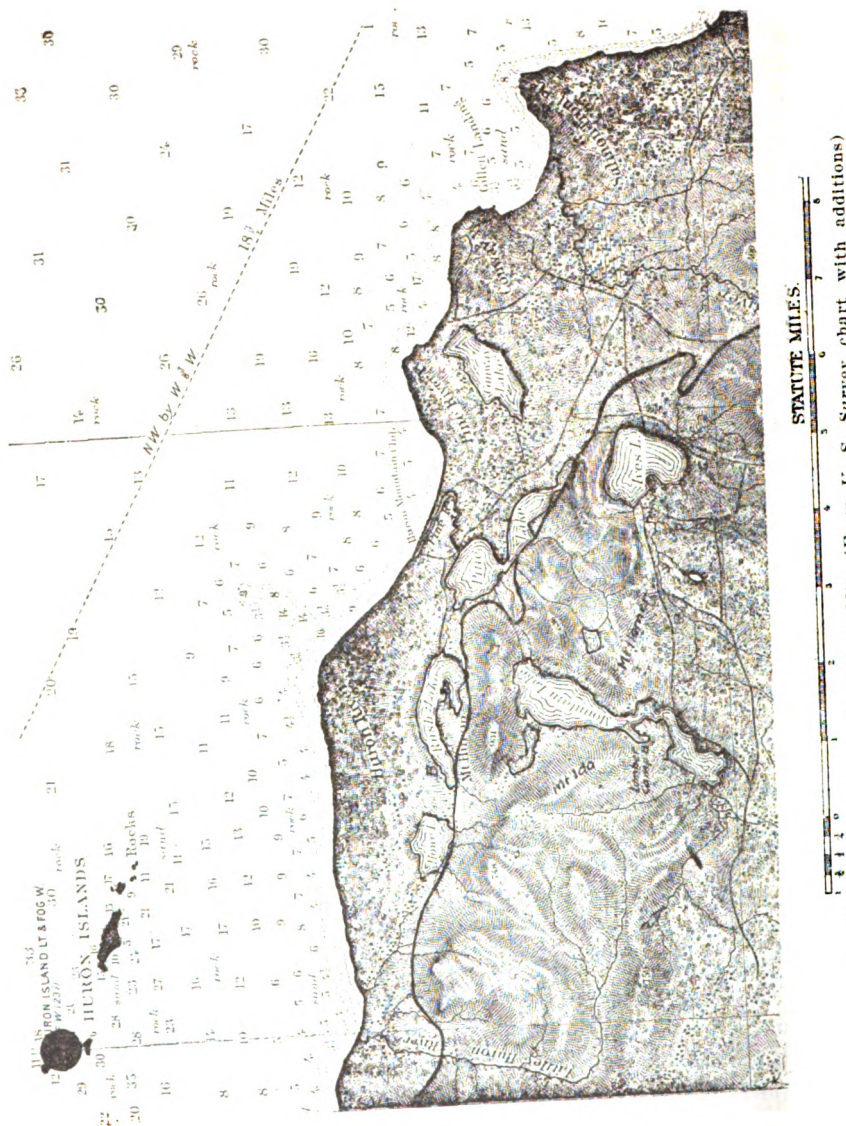
Fig. 84. Relief map of the Huron Mts. (From C. Z. Survey, Ennis with additional data.)
