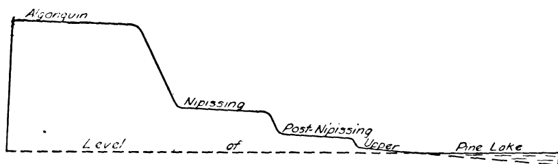
Fig. 53. Diagram showing exposed terraces along the shores of Pine Lake.
