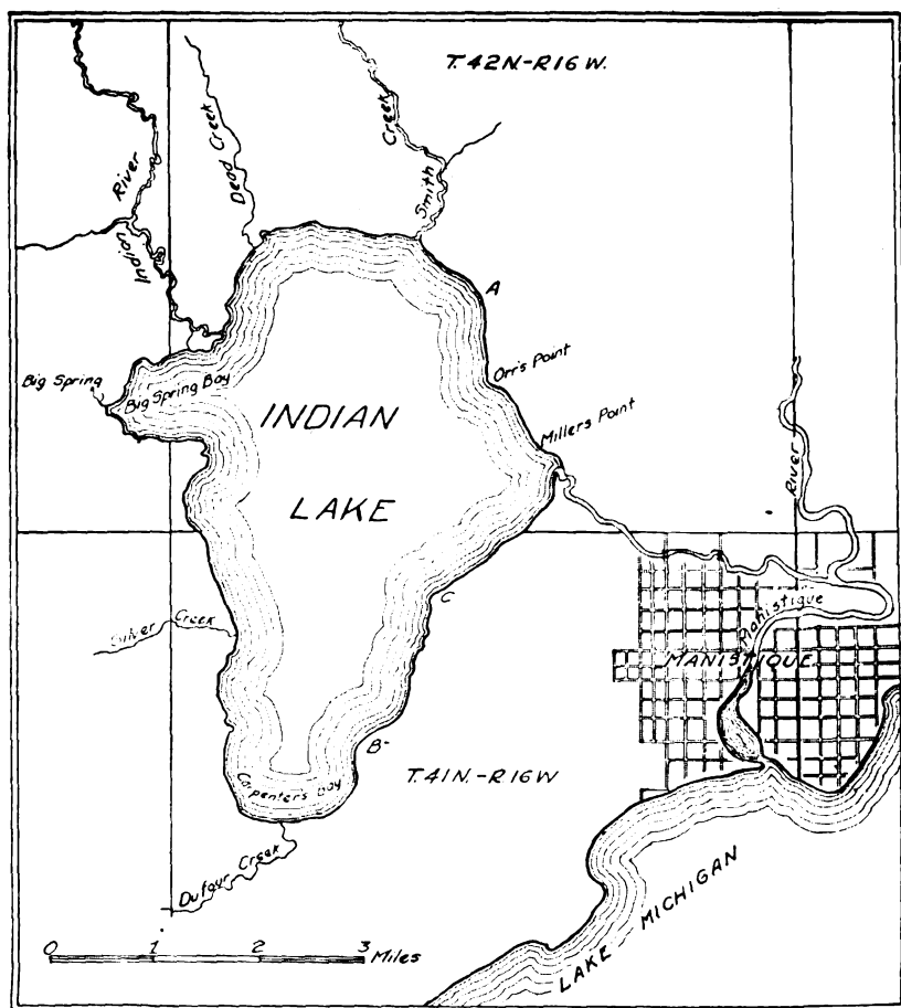
Fig. S3. Outline map of Indian Lake near Mantstique, Schoolcraft County.
