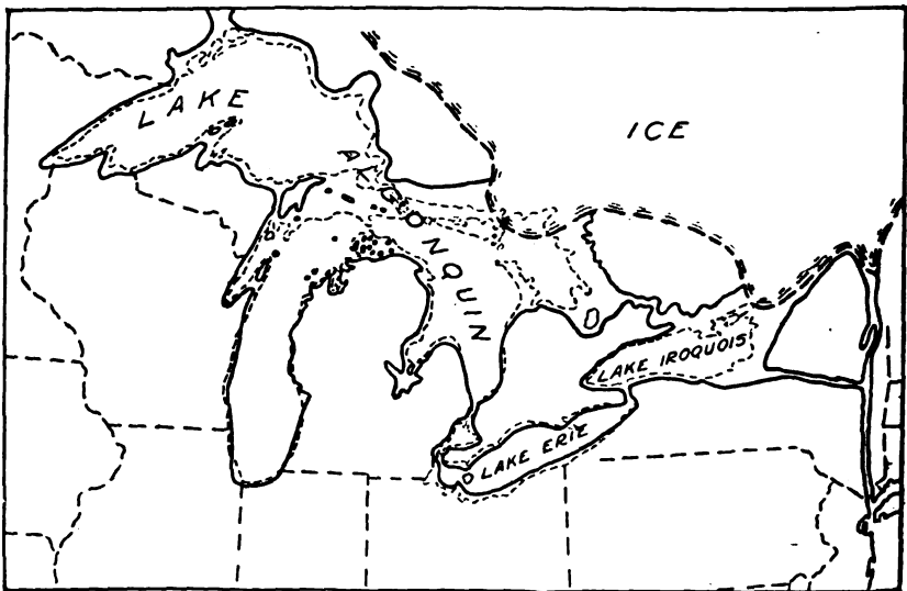
Fig. 4. Map of Lake Algonquin showing relation to present Great Lakes, (after Taylor and Leverett).
