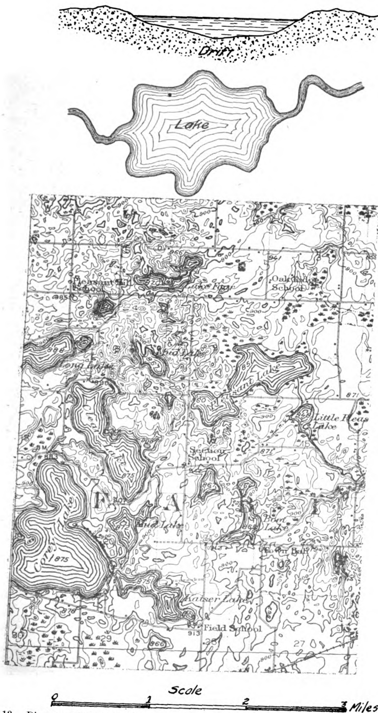
Fig. 12. Diagrams and map showing characteristics of morainal (marginal) lakes. (Diagrams after Hobbs. Map a part of the Three Rivers, Mich., Quadrangle.)
