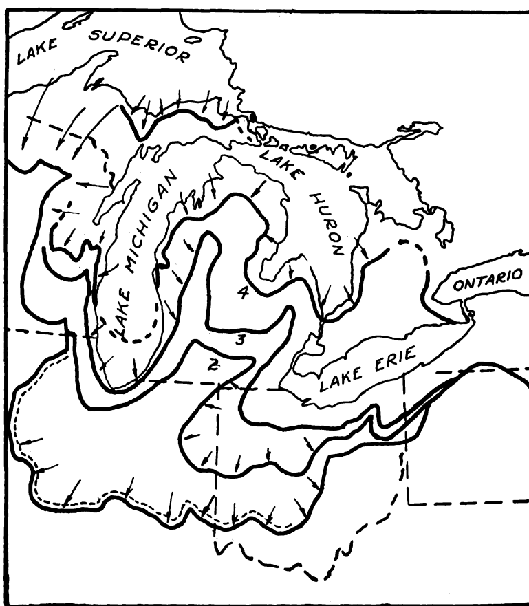
Fig. 3. Map of the principal moranic systems of Michigan. On this map are shown the southern limits of the Wisconsin stage of glaciation; 2, the Kalamazoo-Mississinawa moranic system; 3, the Valparaiso-Charlotte moranic system; 4, Port Huron moranic system.
