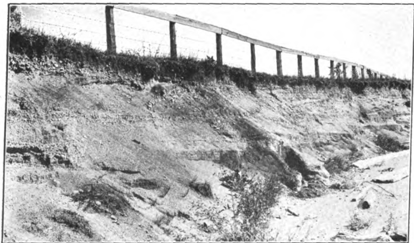
A. STRATIFIED EDGE OF BUILT TERRACE, TORCHLIGHT LAKE.
