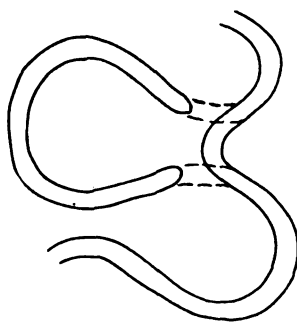
Fig. 8. Map and diagrams showing characteristics of oxbow lakes. Map a part of the Ypsilanti quadrangle.
