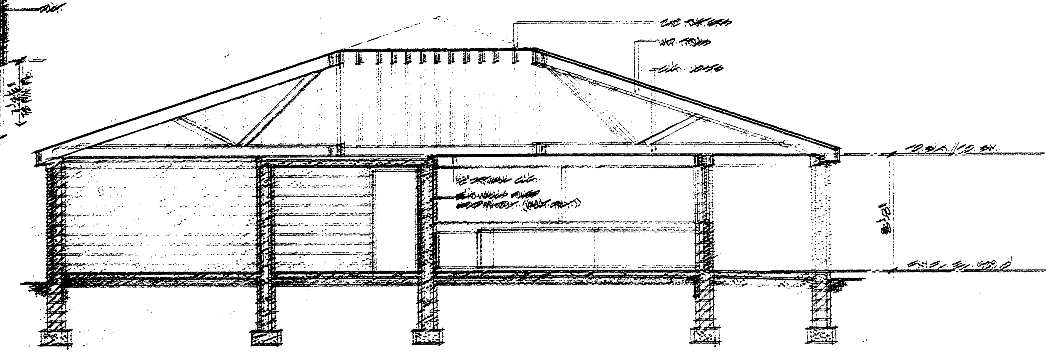
② BUILDING SECTION
